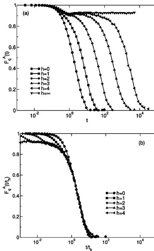
FIG. 6. (a) The dynamic structure factor at q\sigma_{BB}=6.37 for the state point \phi=0.52 , T=0.5 (see Fig. 1) for various values of the barrier height h . The attractive plateau persists longer as h increases, i.e., as the bond lifetime is increased. Panel (b) shows that the functions collapse onto a common curve at long times, when t is rescaled (see text).
