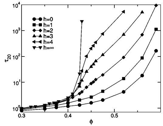
FIG. 8. The dependence of \tau_{20} on h and \phi , obtained from F_q^A(t) at q\sigma_{BB}=2\pi . The curves are for h=0 (circles), h=1 (squares), h=2 (diamonds), h=3 (up triangles), h=4 (left triangles), and permanent bonds (down triangles). For permanent bonds, \tau_{20} diverges near \phi=0.43 . For smaller values of h , \tau_{20} at smaller \phi tracks the divergence at \phi=0.43 , but then crosses over to glassy dynamics with a divergence at higher \phi .
