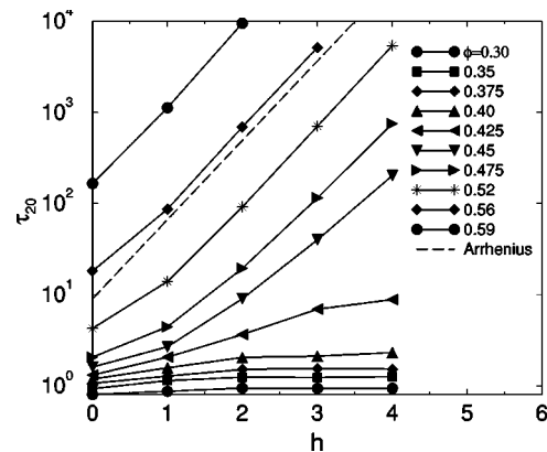
FIG. 9. The dependence of \tau_{20} on h for various packing fractions, at q\sigma_{BB}=2\pi . Above \phi_c , the characteristic time tends to an Arrhenius behavior with h , i.e., \tau_{20} \approx \exp(h/T) .
