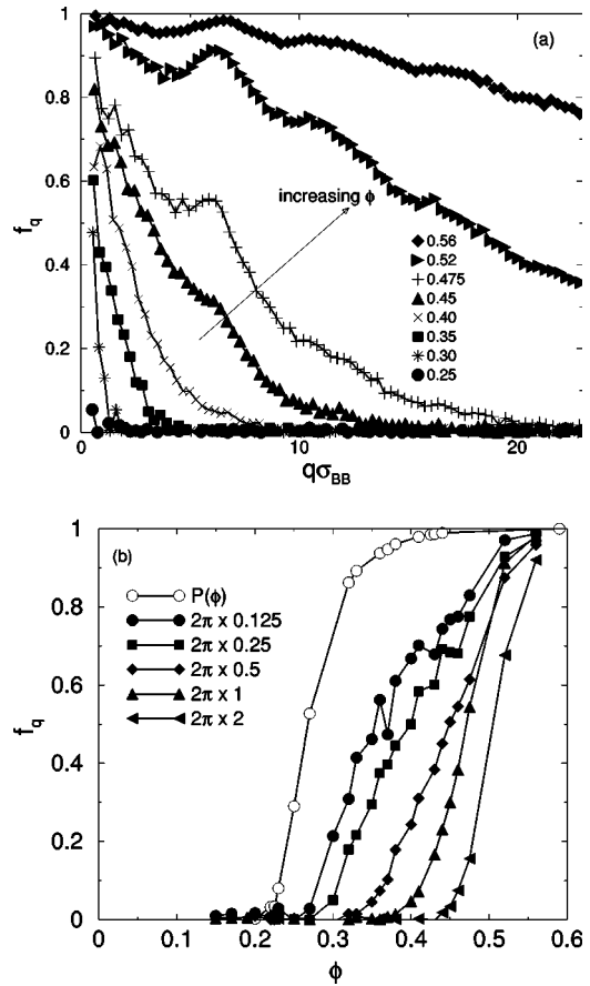
FIG. 5. (a) Plateau height f_q as a function of q for various \phi , for infinite h (irreversible permanent bonds). Legend gives \phi values. (b) Connection to percolation: f_q as a function of \phi for various q . The legend indicates values of q\sigma_{BB} for f_q curves corresponding to filled symbols. The curve labeled with open circles shows P , the average fraction of particles participating in a percolating cluster (taken from Fig. 3).
